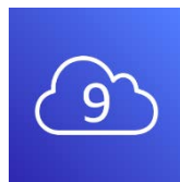
AWS Cloud9
