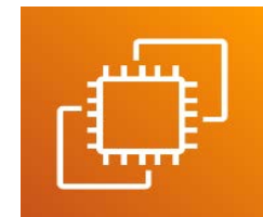
Amazon EC2
