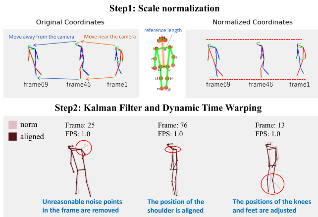
Figure 1: Schematic of motion data preprocessing procedures
