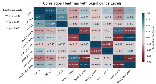
Figure 2: Correlateion analyze
