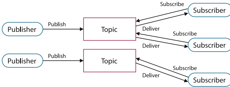
Fig. 1. A conceptual diagram of Pub/Sub
