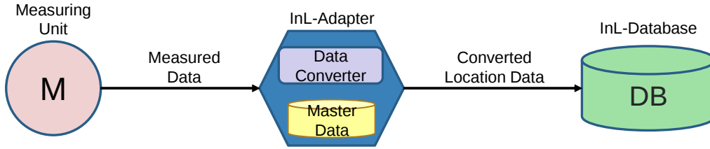
Fig. 2.7. Configuration of InL-Adapter
