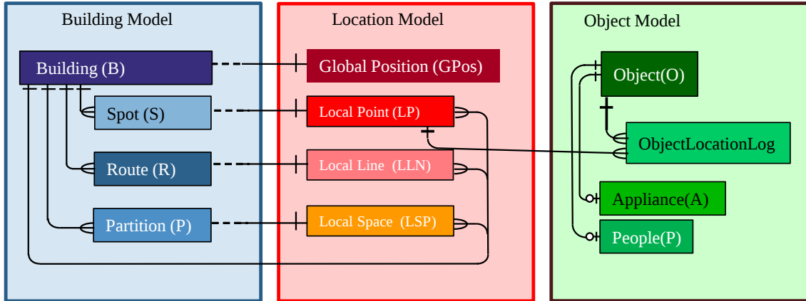
Fig. 2.5. DM4InL as A Composition of Three Models
