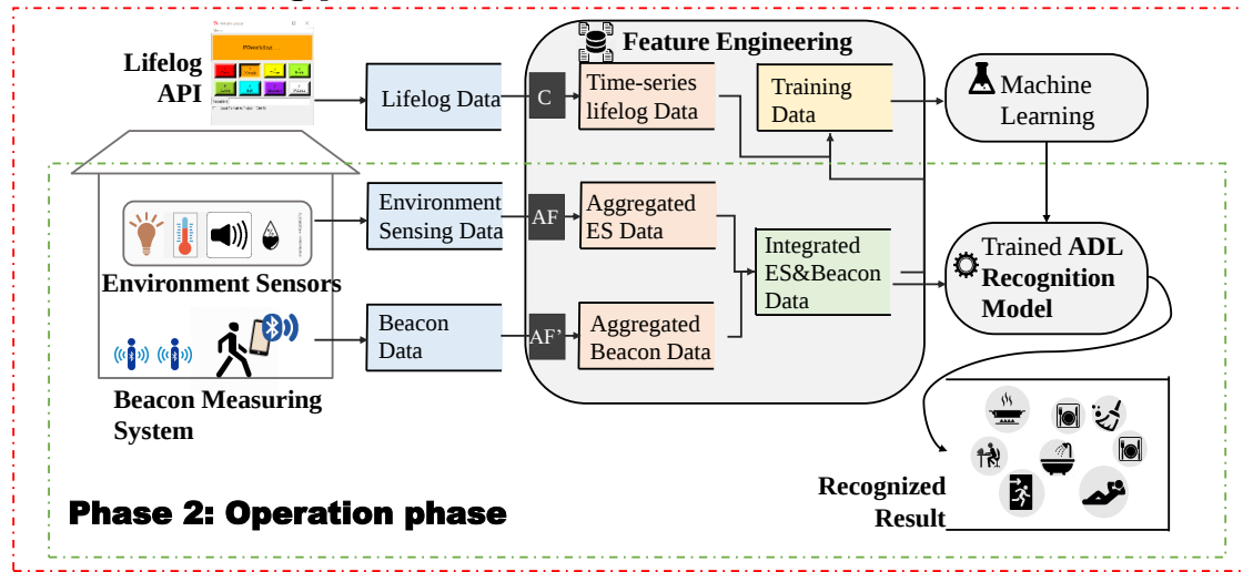
Fig. 3.9. Architecture of Proposed System
