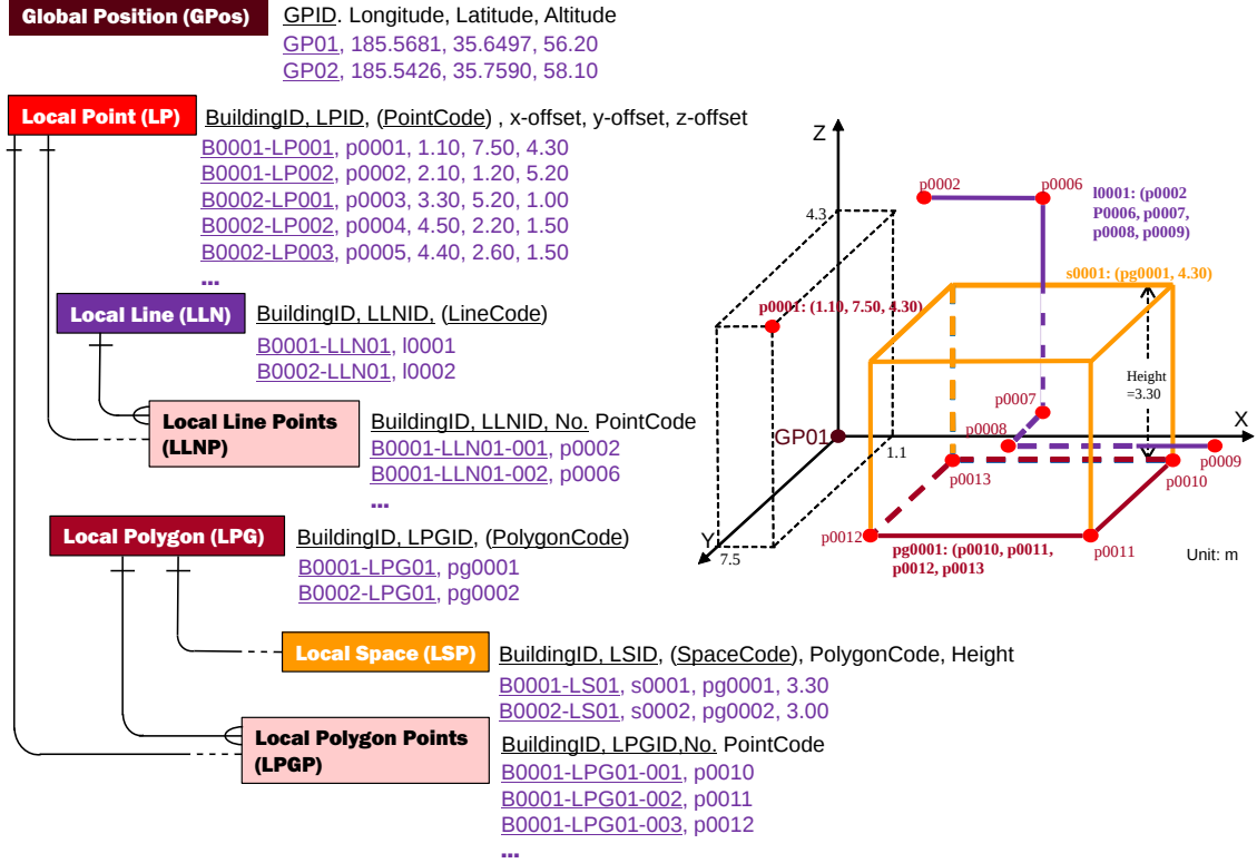
Fig. 2.2. Entity Relationship (ER) Diagram of Location Model and Schematic Representations of Instances
